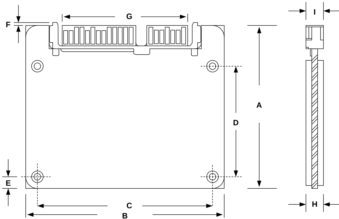
Figure 2: Physical Dimensions
