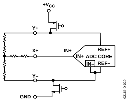
Figure 29. Differential Reference Mode ( SER/\overline{DFR} = 0 )
