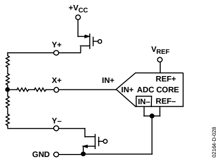
Figure 28. Single-Ended Reference Mode ( SER/\overline{DFR} = 1 )
