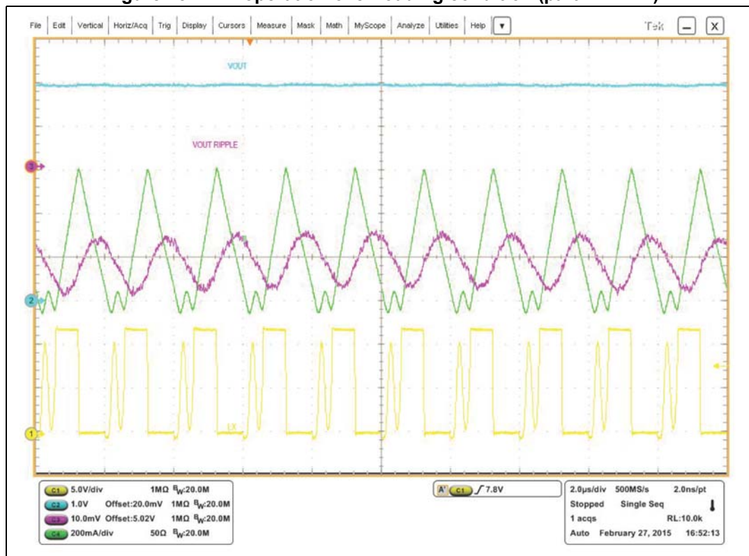
Figure 26. LCM operation over loading condition (part 5 - CCM)
