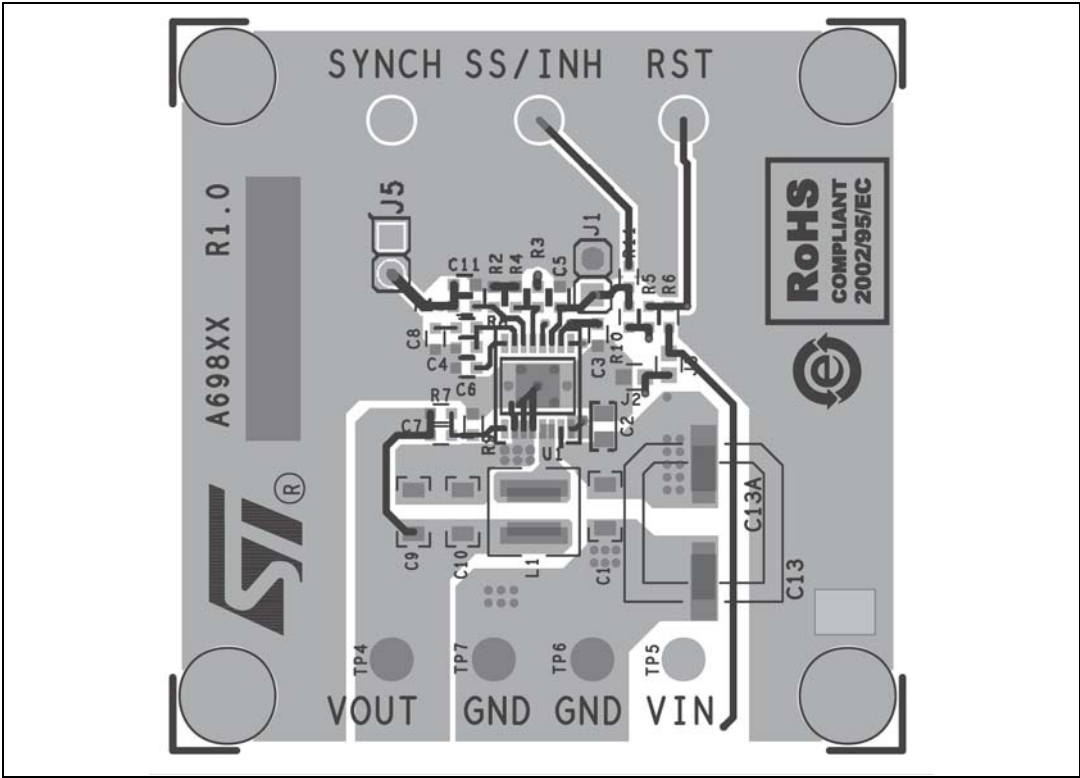
Figure 55. Top layer
