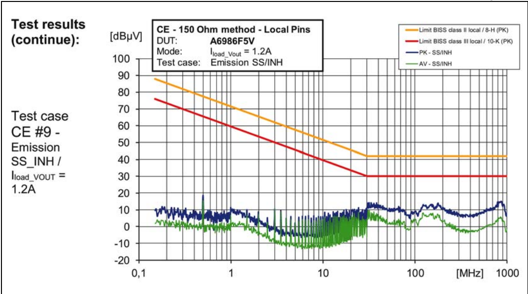
Figure 72. CE 150R at SS/INH test point (see Figure 65 on page 70) at 80% I LOAD
