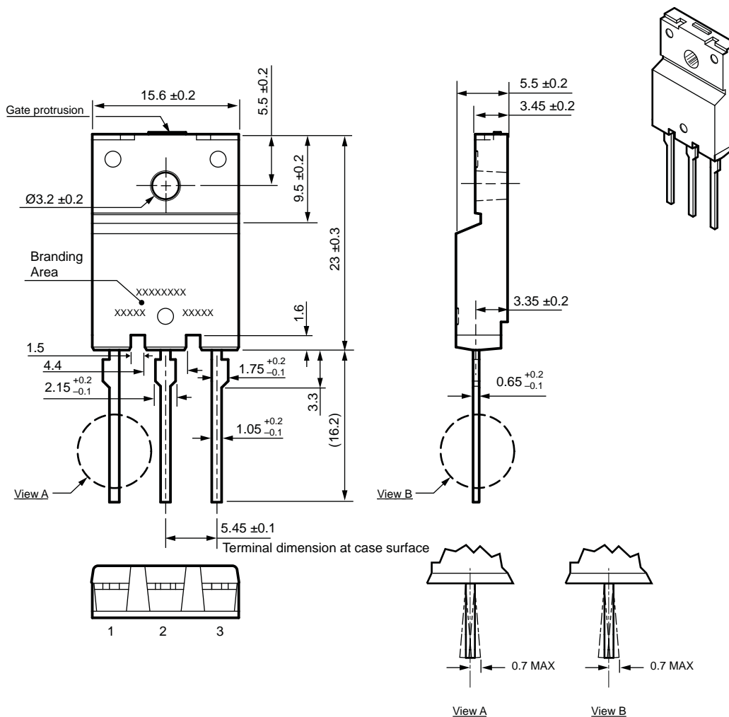
TO-3PF Package Outline Drawing
