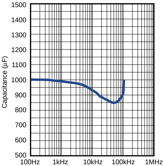
TYPICAL CAP FREQUENCY SCAN @ 25°C T510E108M004AS
