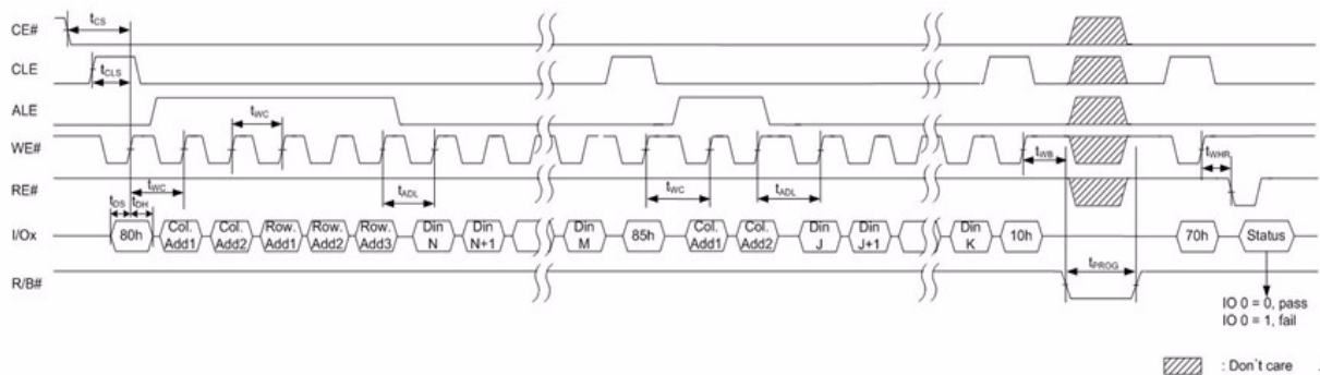
■ Figure 24. Random data input timings
