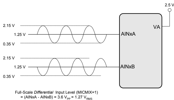
Figure 9. Differential Input
