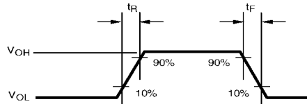
FIGURE 1. Rise and Fall Times
