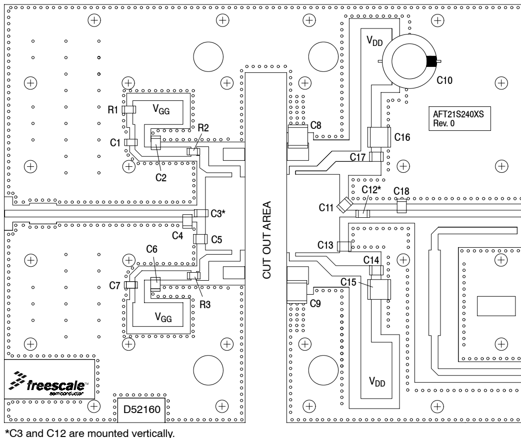
Figure 3. AFT21S240-12SR3 Characterization Test Circuit Component Layout
