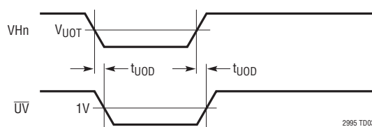
VHn Monitor Timing (TMR Pin Strapped to V CC )
