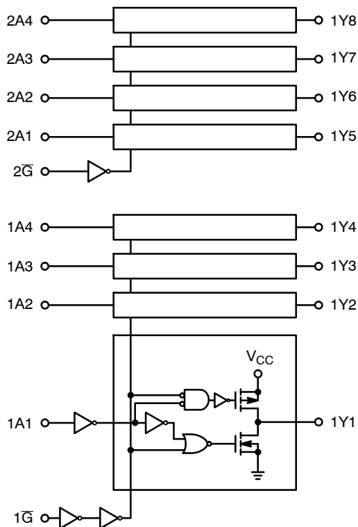
Figure 1. Logic Diagram
