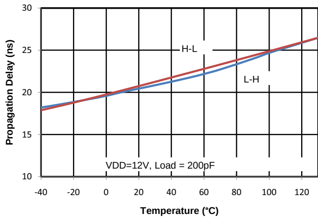
Figure 30. Propagation Delay vs. Temperature
