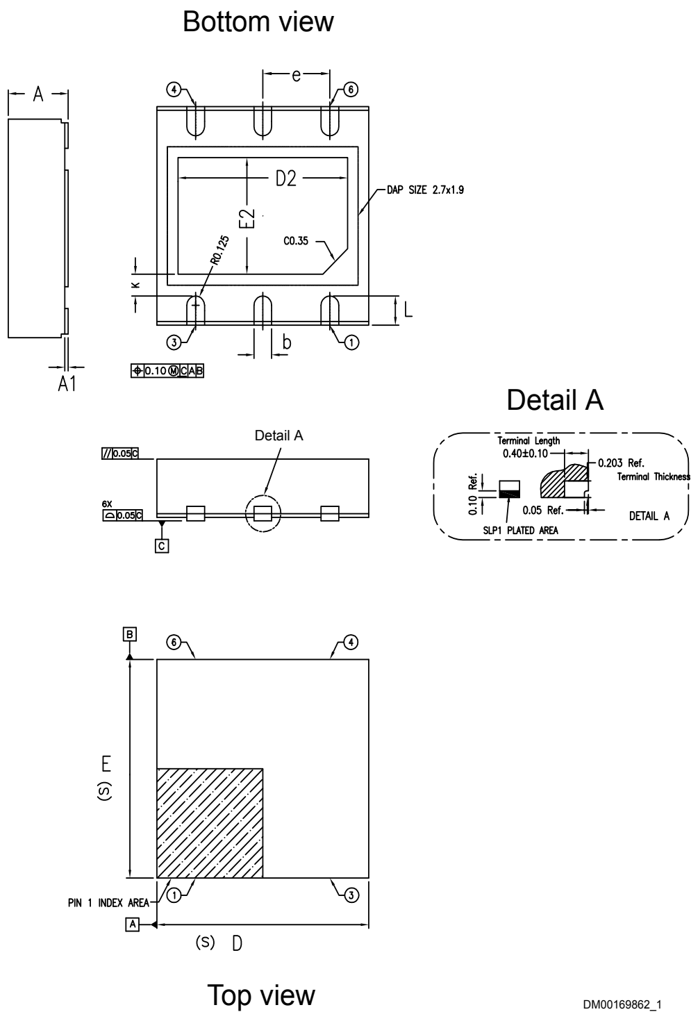
Figure 35. DFN6 (3x3 mm) automotive-grade package outline
