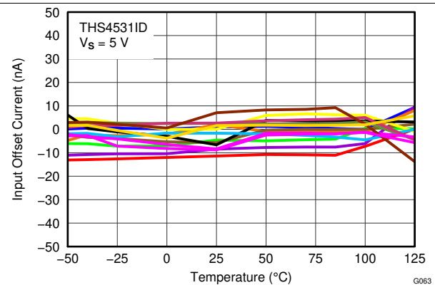
Figure 64. Input Offset Current vs Temperature
