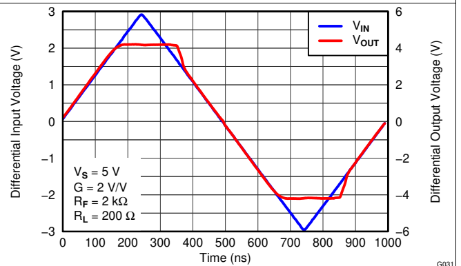
Figure 40. Overdrive Recovery
