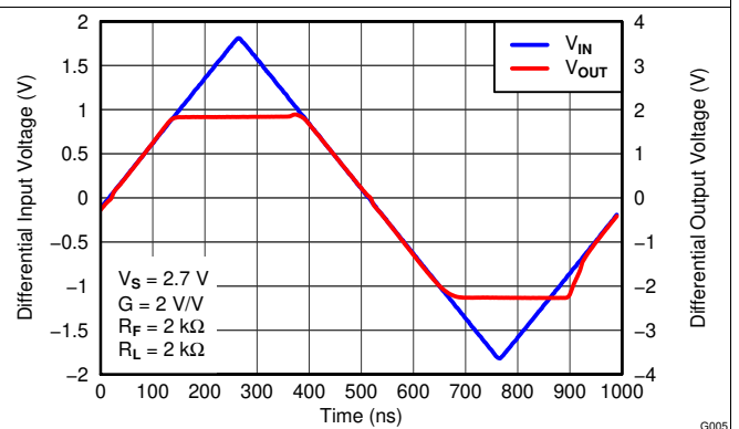
Figure 7. Overdrive Recovery
