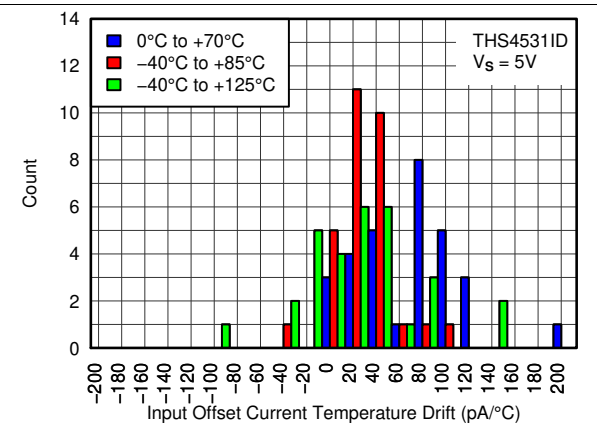
Figure 63. Input Offset Current Temperature Drift Histogram
