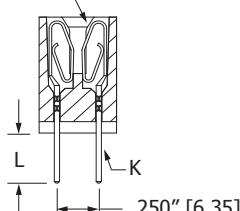
LOOP BELLOWS (TK,RS,RM,CK)
