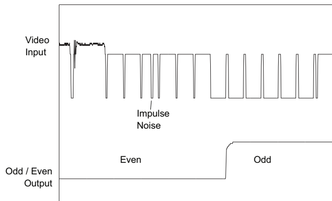
Figure 2-4: Noise Immunity of Odd/Even Output
