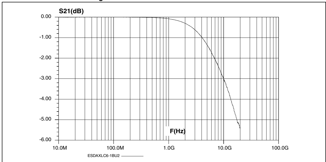
Figure 7. Attenuation measurement results
