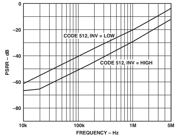
TPC 18. AVCC Power Supply Rejection vs. Frequency
