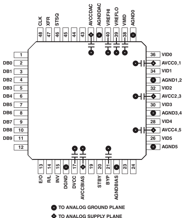
Figure 11. AD8381 Recommended Bypassing
