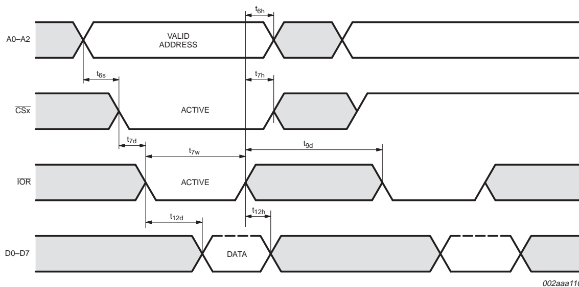
Fig 8. General read timing.
