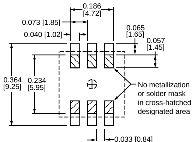
Suggested PCB Pad Layout
