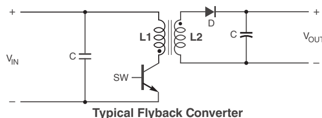
Typical Flyback Converter
