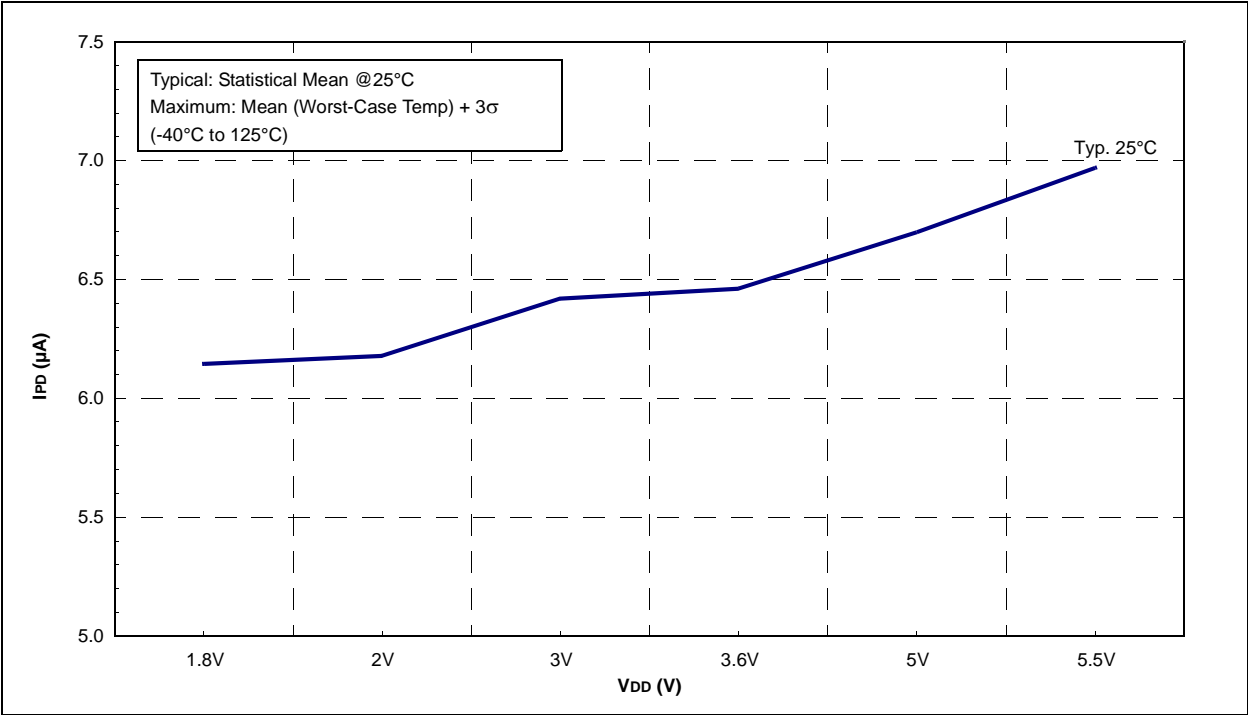
FIGURE 26-43: PIC16F707 TYPICAL ADC I_{PD} vs. V DD , V CAP = 0.1 \mu F
