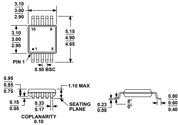
Figure 53. 10-Lead Mini Small Outline Package [MSOP] (RM-10)
