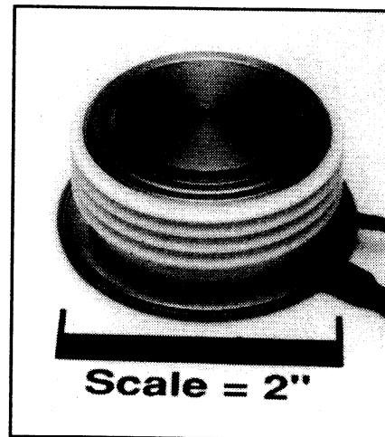
C441 Phase Control SCR 750 Amperes Average, 2400 Volts
