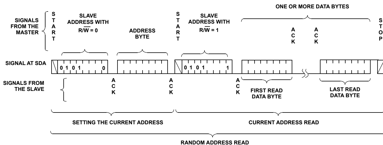
FIGURE 10. MOVE/READ SEQUENCE
