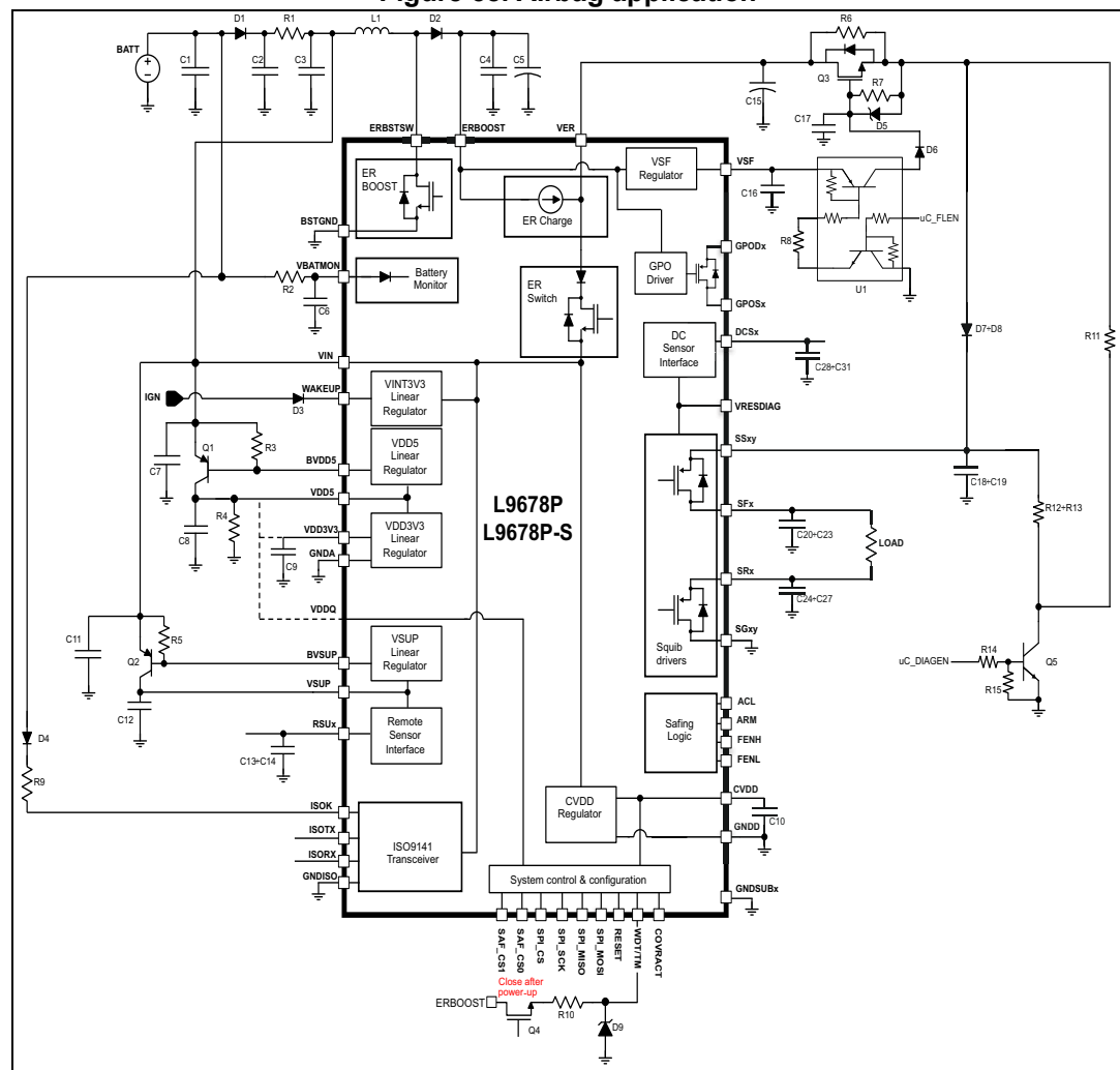
Figure 58. Airbag application
