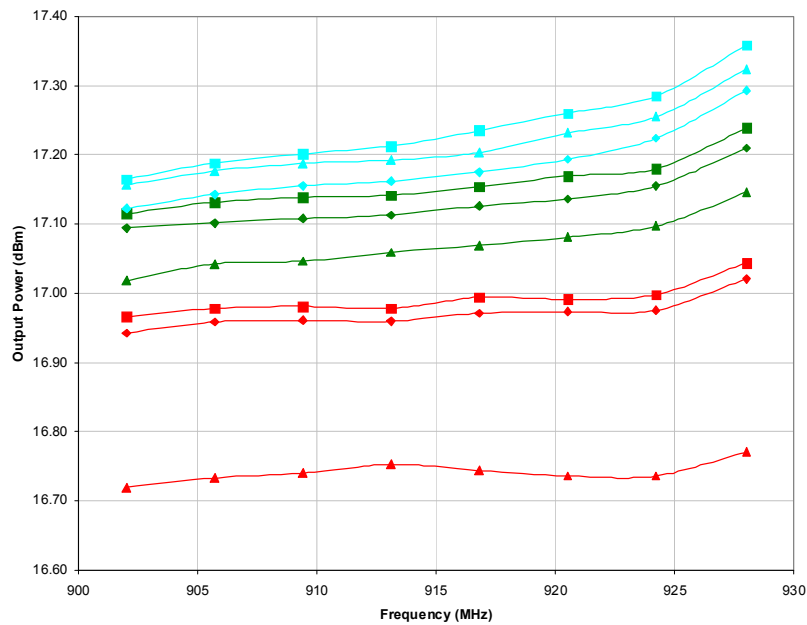
Figure 26. Typical 17 dBm Output Power Flatness versus Supply Voltage and Temperature, Measured in the 915 MHz ISM band
