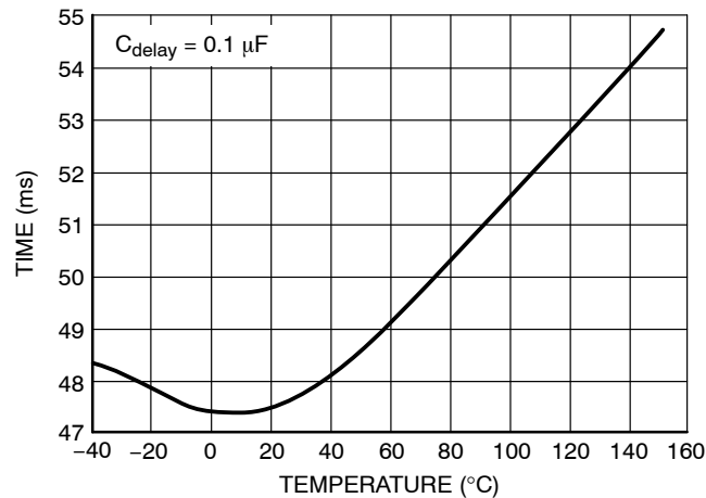
Figure 6. Delay Time
