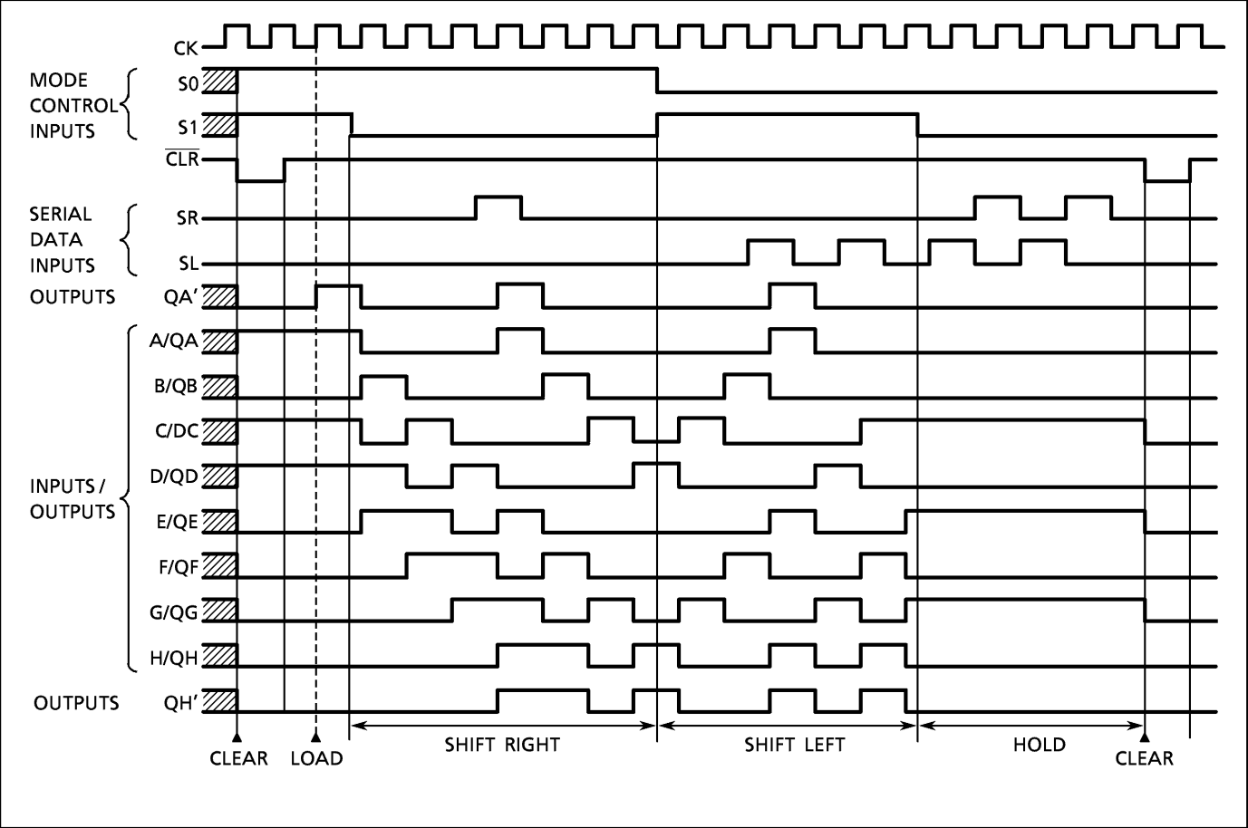
TIMING CHART
