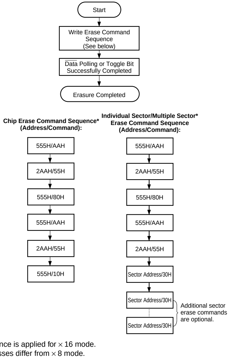
Figure 23 Embedded Erase™ Algorithm
