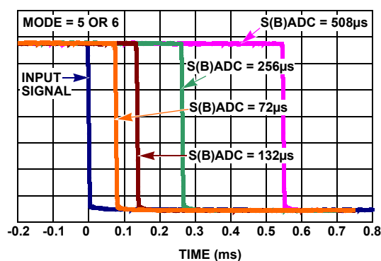
FIGURE 26. INTERRUPT TIMING
