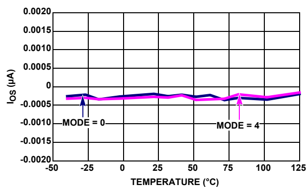
FIGURE 22. SHUNT I_{OS} vs TEMPERATURE (MODE 0, 4)
