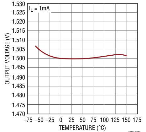
LT3060-1.5 Output Voltage
