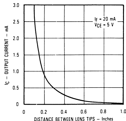
Coupling Characteristics of OP168F and OP538F
