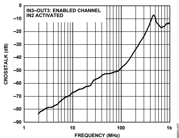
Figure 34. ADV3227 Crosstalk, One Adjacent Channel, RTO
