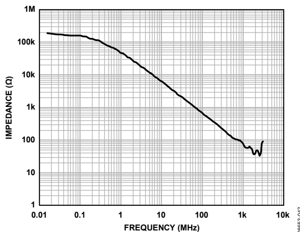
Figure 36. ADV3227 Input Impedance
