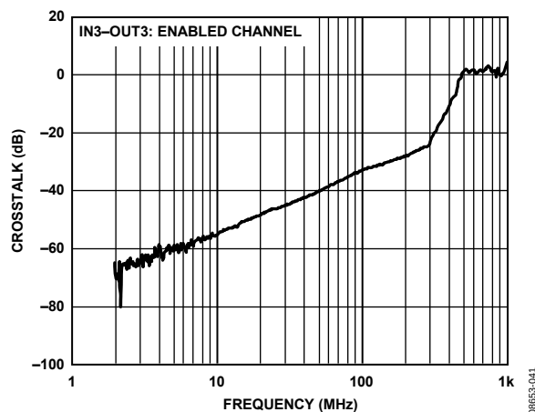
Figure 35. ADV3227 Crosstalk, All Hostile, RTO
