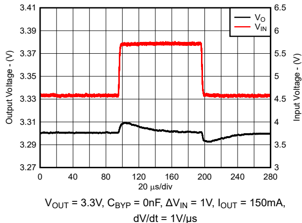
Figure 5-46. Line Transient Response (New Chip)
