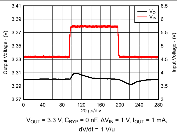
Figure 7-8. Line Transient Response for New Chip
