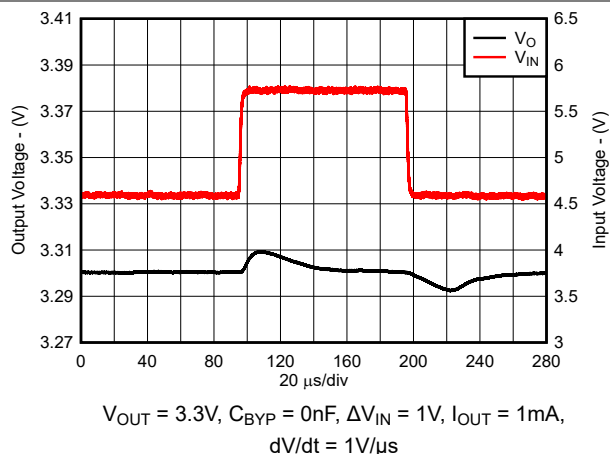
Figure 5-44. Line Transient Response (New Chip)
