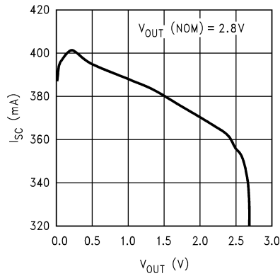
Figure 5-7. Short-Circuit Current vs Output Voltage (Legacy Chip)
