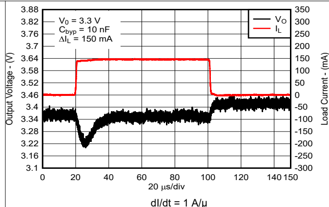
Figure 7-4. Load Transient for New Chip
