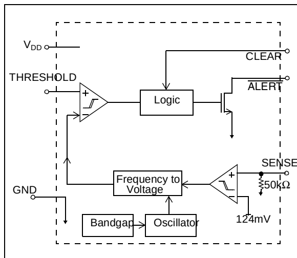
FIGURE 4-1: TC670 BLOCK DIAGRAM
