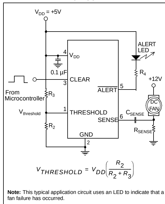
FIGURE 4-2: TYPICAL APPLICATION CIRCUIT
