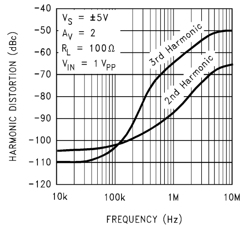
Harmonic Distortion vs. Frequency (Note 13)
