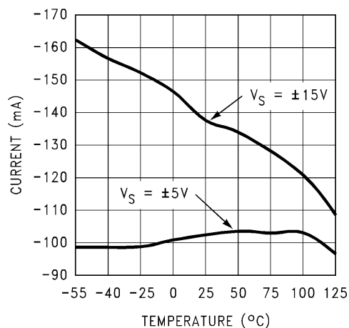
Short Circuit Current vs. Temperature (Sinking)
