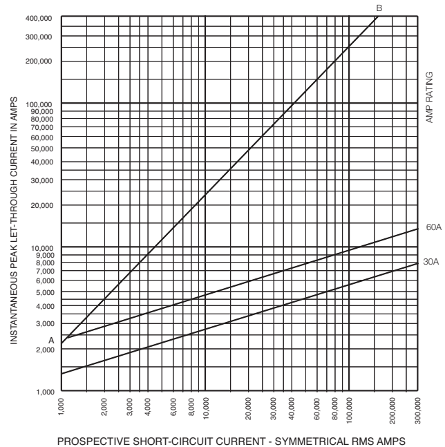
Current-Limiting Effects
