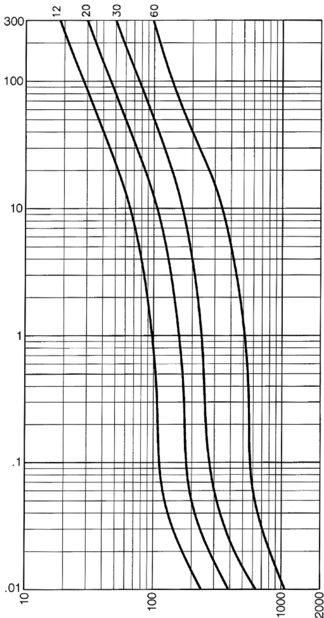
Time-Current Characteristic Curves—Average Melt 12 to 60 Amps
