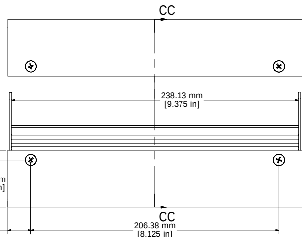
ASSEMBLY - VIEW FROM SIDE (OPEN)
