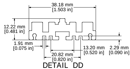
END PLATE - VIEW FROM OUTSIDE
