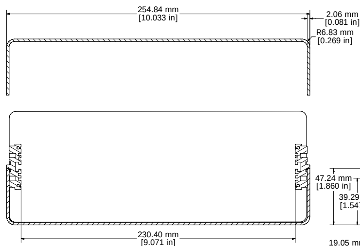
SECTION CC-CC
