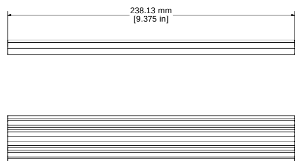
EXTRUSION - VIEW FROM INSIDE
