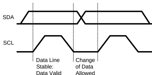
Figure 15. Bit Transfer
