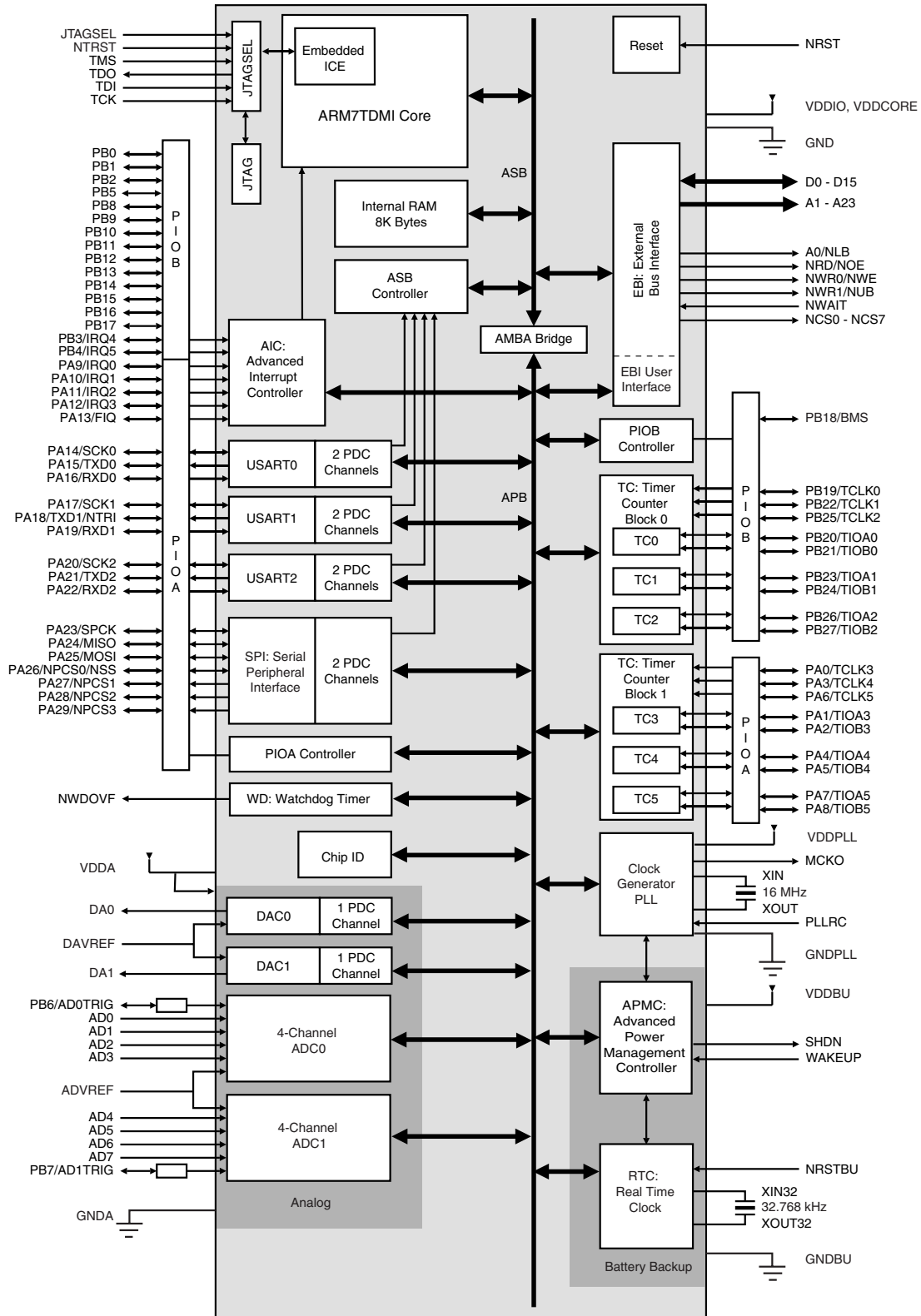
Figure 4-1. AT91M55800A
