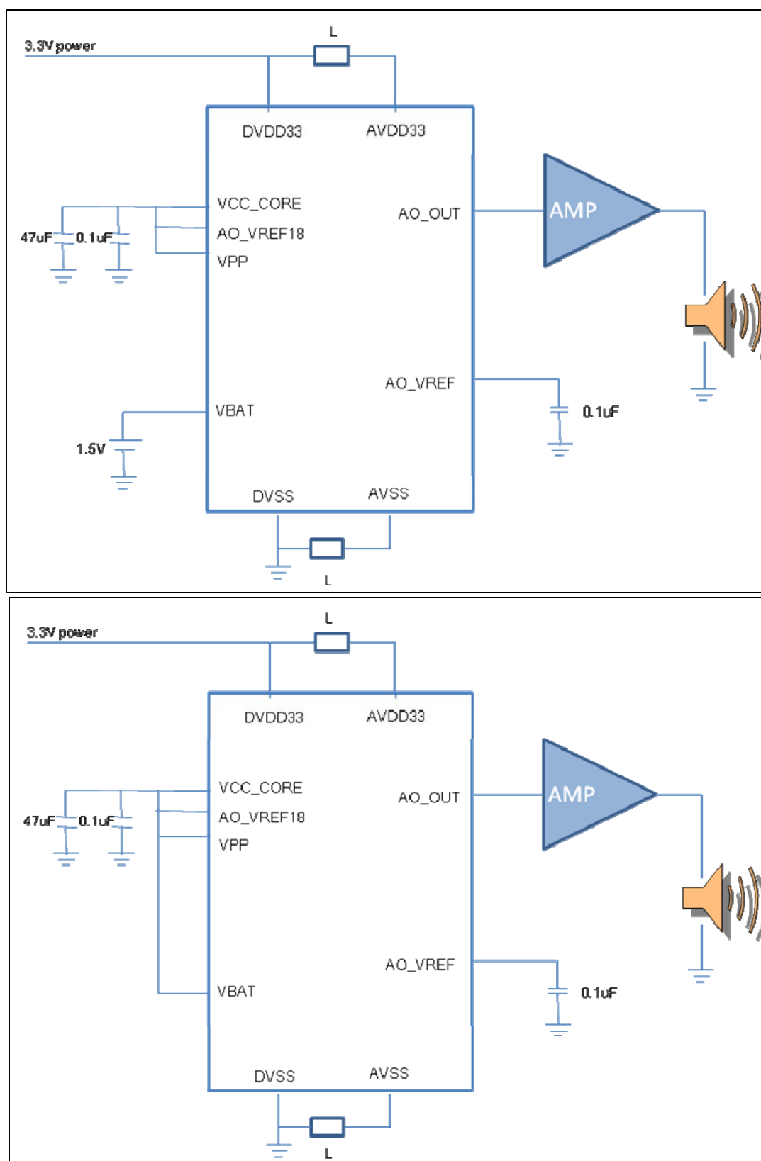
Fig. 15 Connections @ Digital / Analog Power Pins
