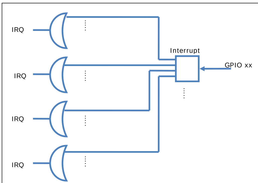
Fig. 13 GPIO Interrupt Block Diagram
