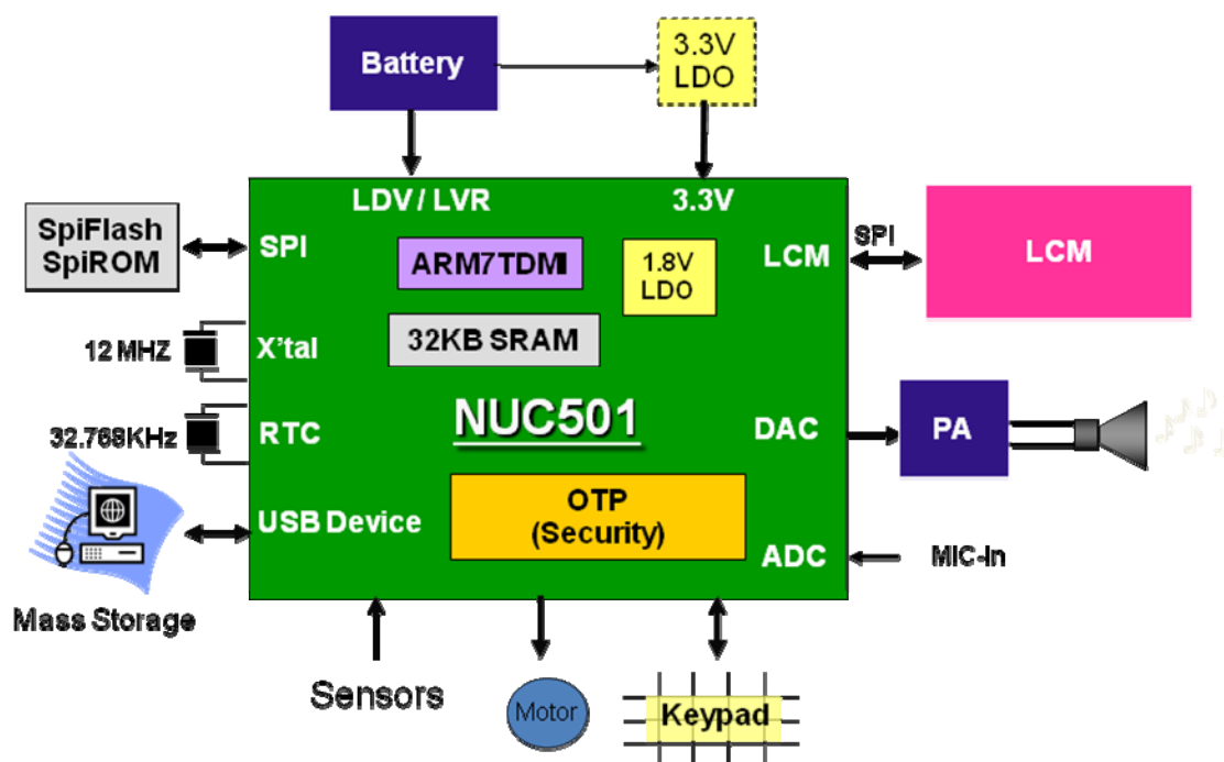
Fig. 3 System Block Diagram
