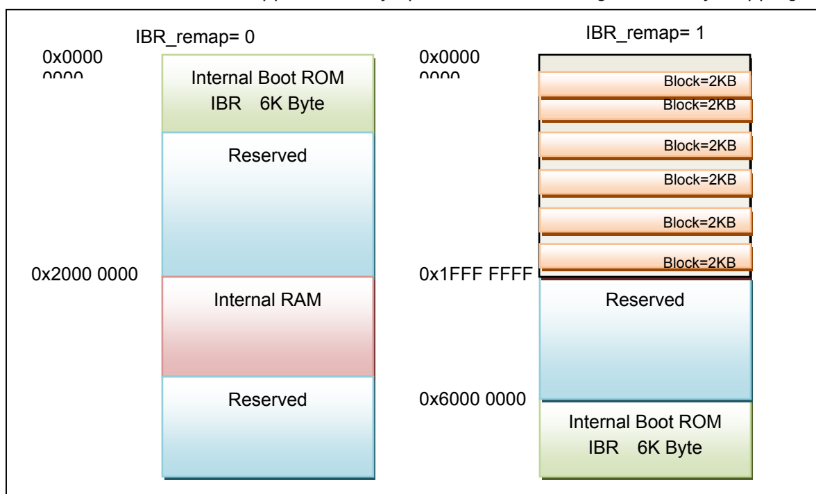
Fig. 5 Memory Mapping
