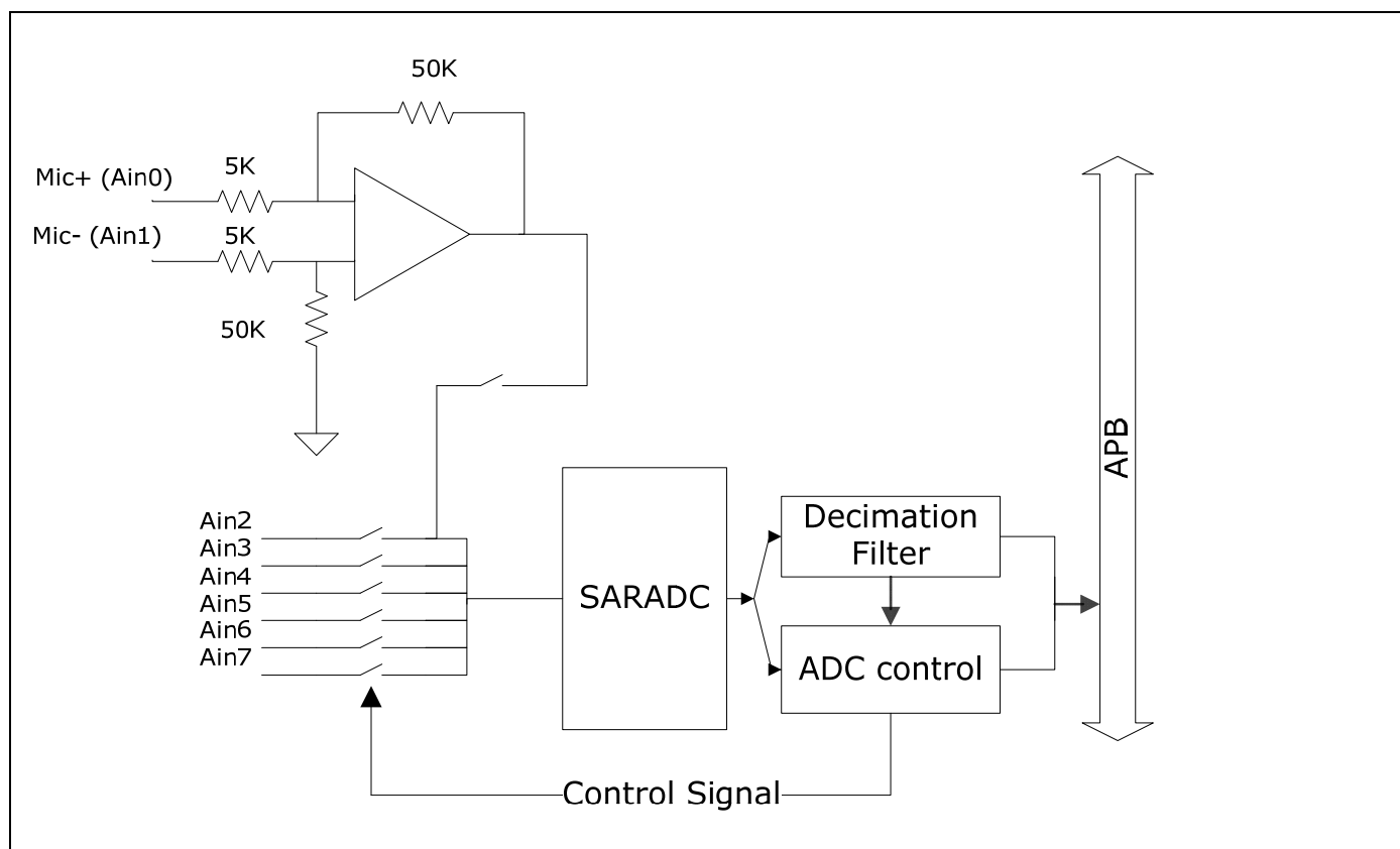
Fig. 8 SAR ADC Block Diagram
