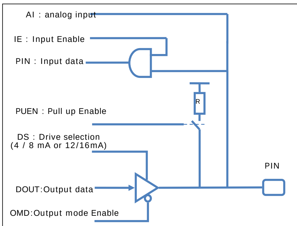
Fig. 12 GPIO Block Diagram
