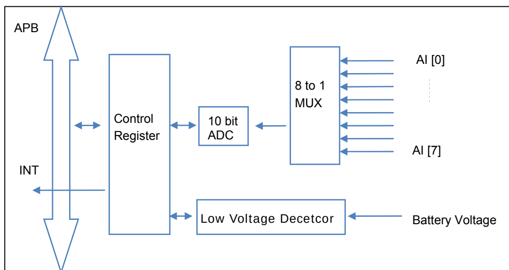
Fig. 6 ADC Block Diagram
