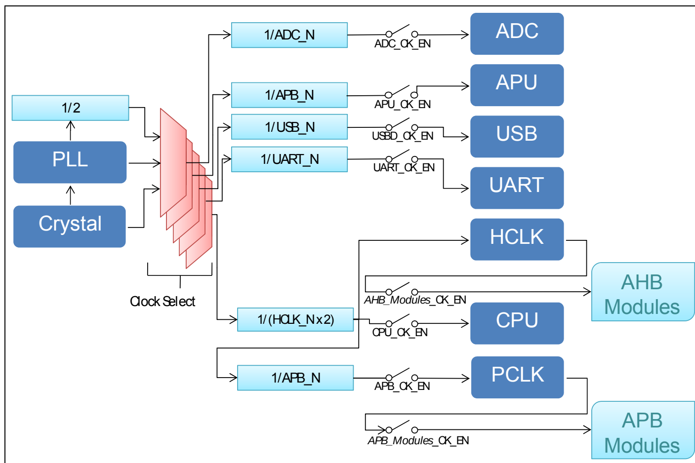
Fig. 9 Clock Controller Block Diagram
