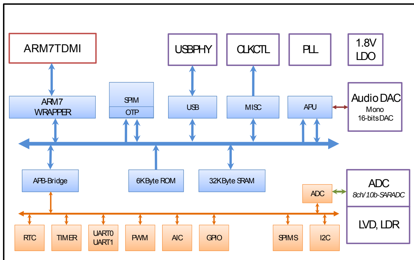
Fig. 4 Block Diagram
