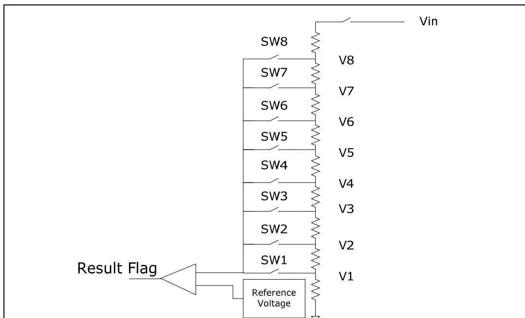
Fig. 7 Architecture of Voltage Detector
