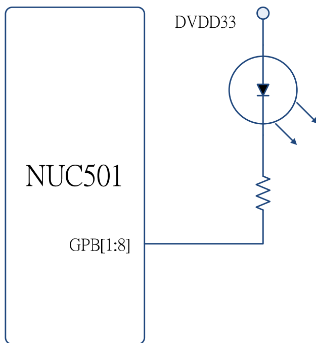
Fig. 16 Direct Sink I/O for LED
