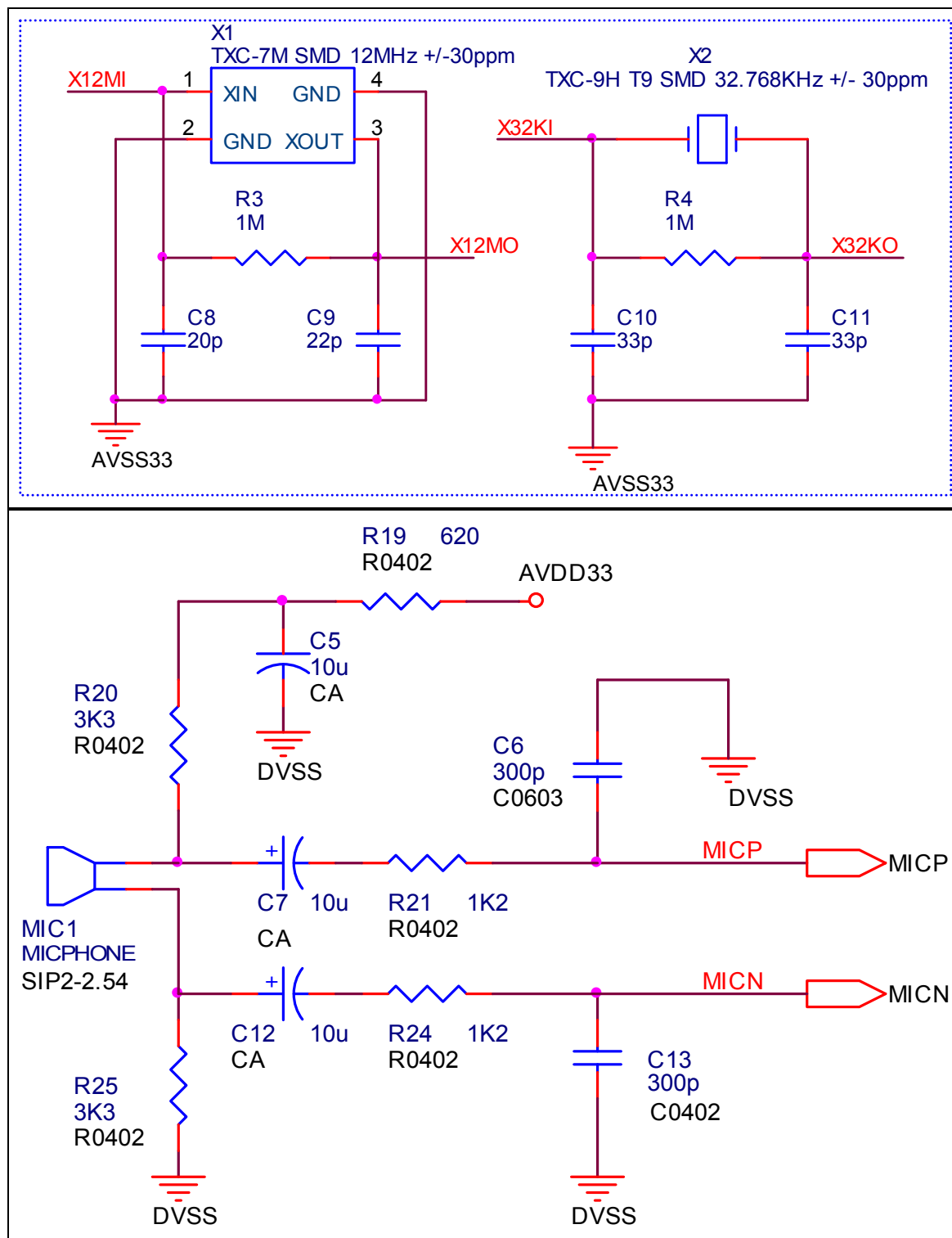
Fig. 14 Connections @ X'tal & MIC
