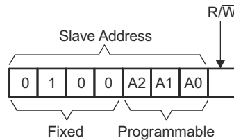
Figure 8-6. PCA9555 Address
