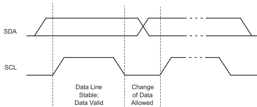
Figure 8-4. Bit Transfer
