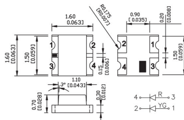
Package Outline Drawing:
