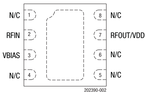
Figure 2. SKY67151-396LF Pinout – 8-Pin DFN (Top View)
