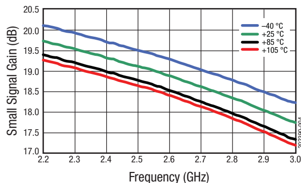
Figure 4. Narrow Band Gain vs Frequency Over Temperature
