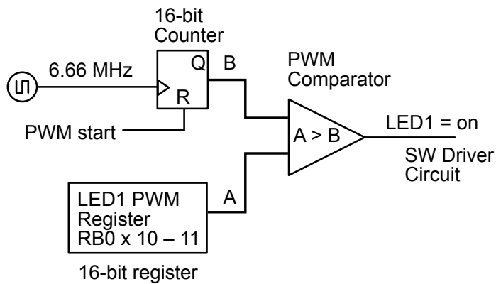
Figure 2: PWM On-time Comparator Circuit
