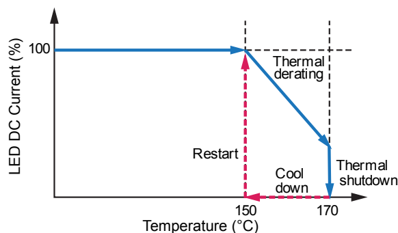
Figure 8: Thermal Derating and Shutdown Protection Features
