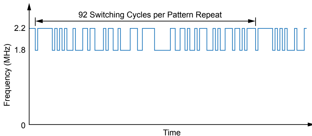
Figure 4: A8517 Dithering Scheme at 2 MHz \pm 10% (frequency jumps between 1.8 MHz and 2.2 MHz, as governed by a 46-bit pseudorandom pattern)
