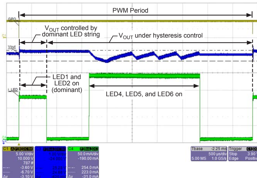
Figure 6: Output Hysteresis Waveform, LED1 and LED2 are the Dominant String
