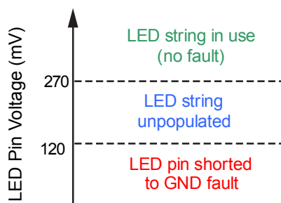
Figure 9: A8517 LED Short-to-GND Check Before Startup
