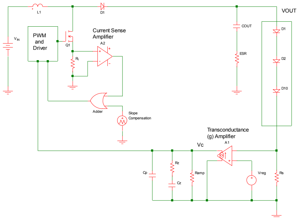
Figure A-2: Small signal model of a peak-current-mode boost converter; the ten strings of the A8517 are represented by one string in this example
