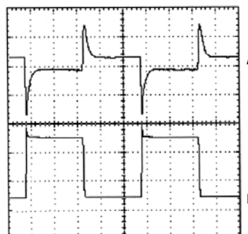
LOAD-TRANSIENT RESPONSE
