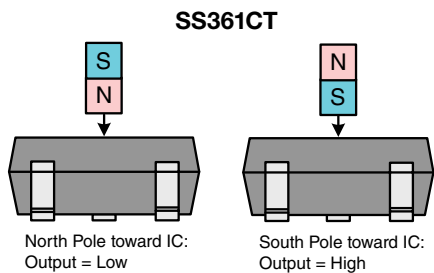
Figure 4. Magnetic Activation
