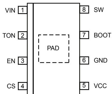
Pinout Diagram
