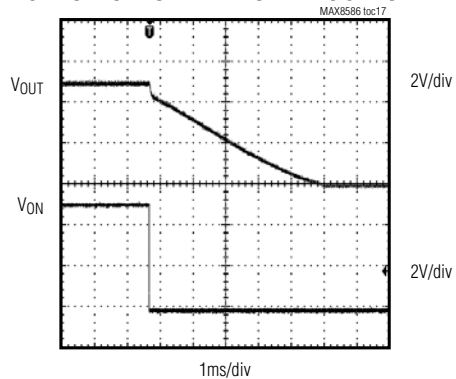
SWITCH TURN-OFF WAVEFORM INTO 5\Omega LOAD
